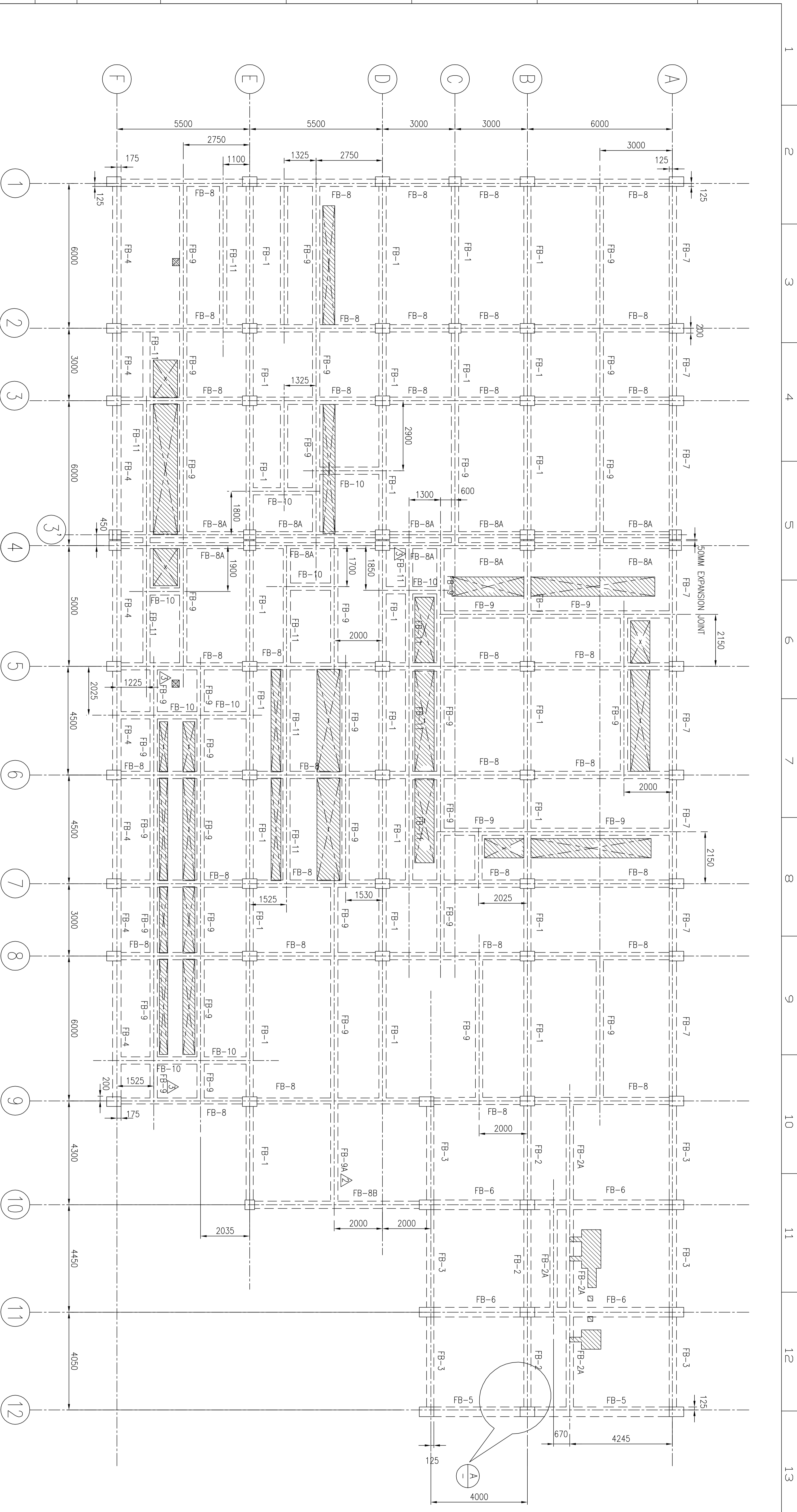
PLAN AT FLOOR BEAM LEVEL [T.O.C. AT EL.(+4.300)]
